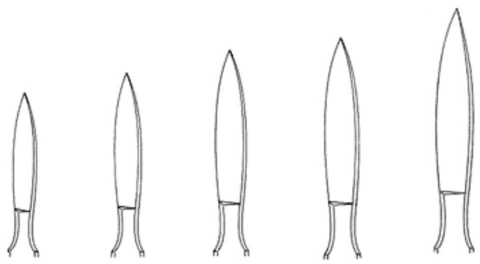
IM-01-06 6" Fig. 6cutting length 27 mm IM-01-07 6" Fig. 7cutting length 35 mm IM-01-08 6 1/4" Fig. 8cutting length 40 mm IM-01-09 6 1/4" Fig. 9cutting length 47 mm IM-01-10 6 3/4" Fig. 10cutting length 50 mm
