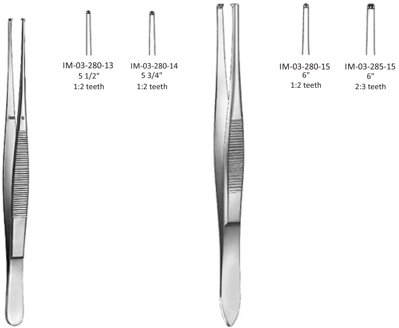
Dissecting Forceps
