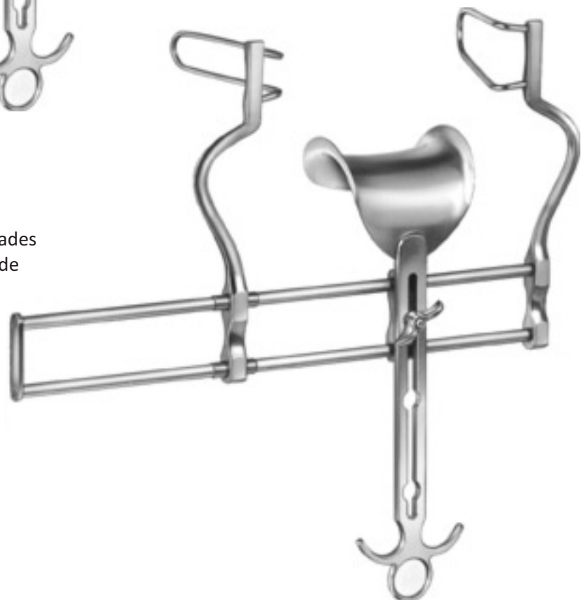
Abdominal Retractor Balfour IM-04-687-00 8" spreading 250 mmlateral blades 100 x 35 mm1 central blade
