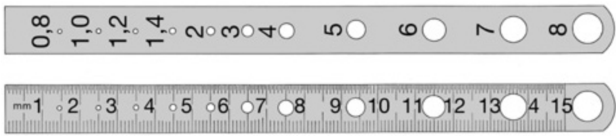
Ruler IM-06-150-15 6 1/2" measuring range up to 150 mm with hole gauge
